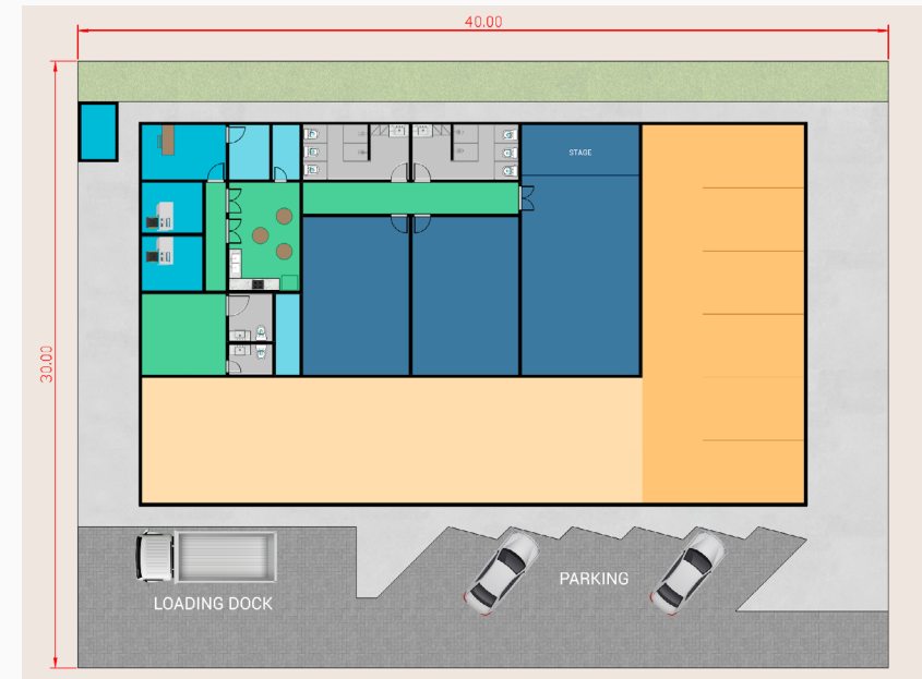
FIGURE 8 Circularity Support Hub floorplan
